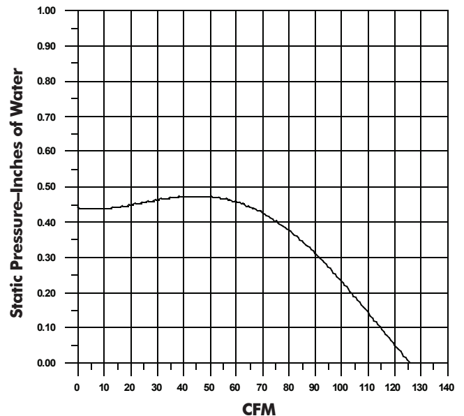
NuVent Product Performance Model NXMR110L
